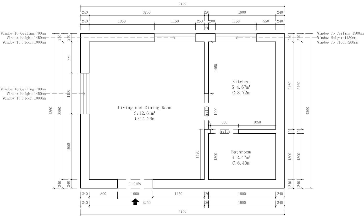
Floor Plan 1:50
